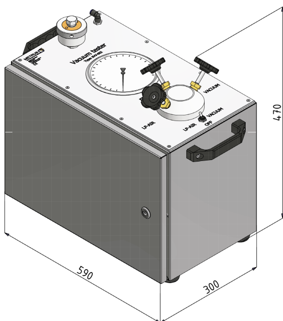
Abmessungen in mm All dimensions in mm
