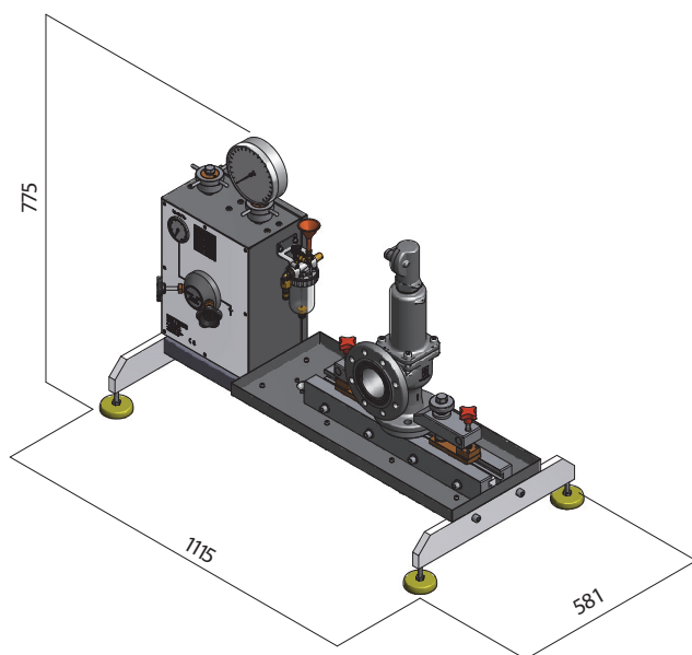
SVM 4/100 DN15-DN100 3/8"-4" basic model
